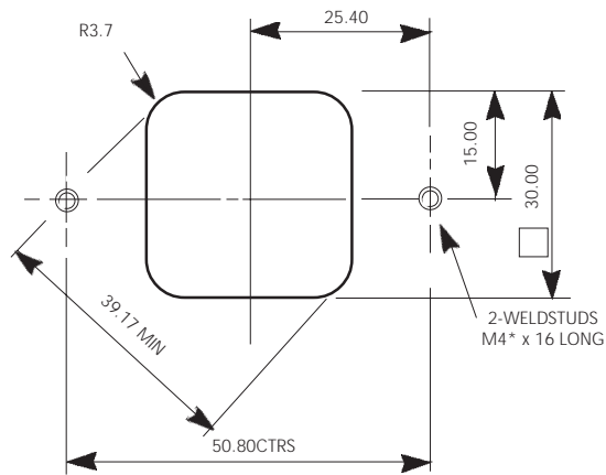
US94 Compact 2 Cutout
